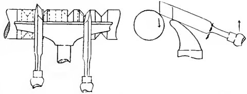
FIG. 309. DETAIL OF CUTTING V-GROOVES.
